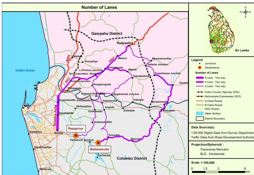
Figure 03: Geometric capacities of BL – road and that of alternative links
